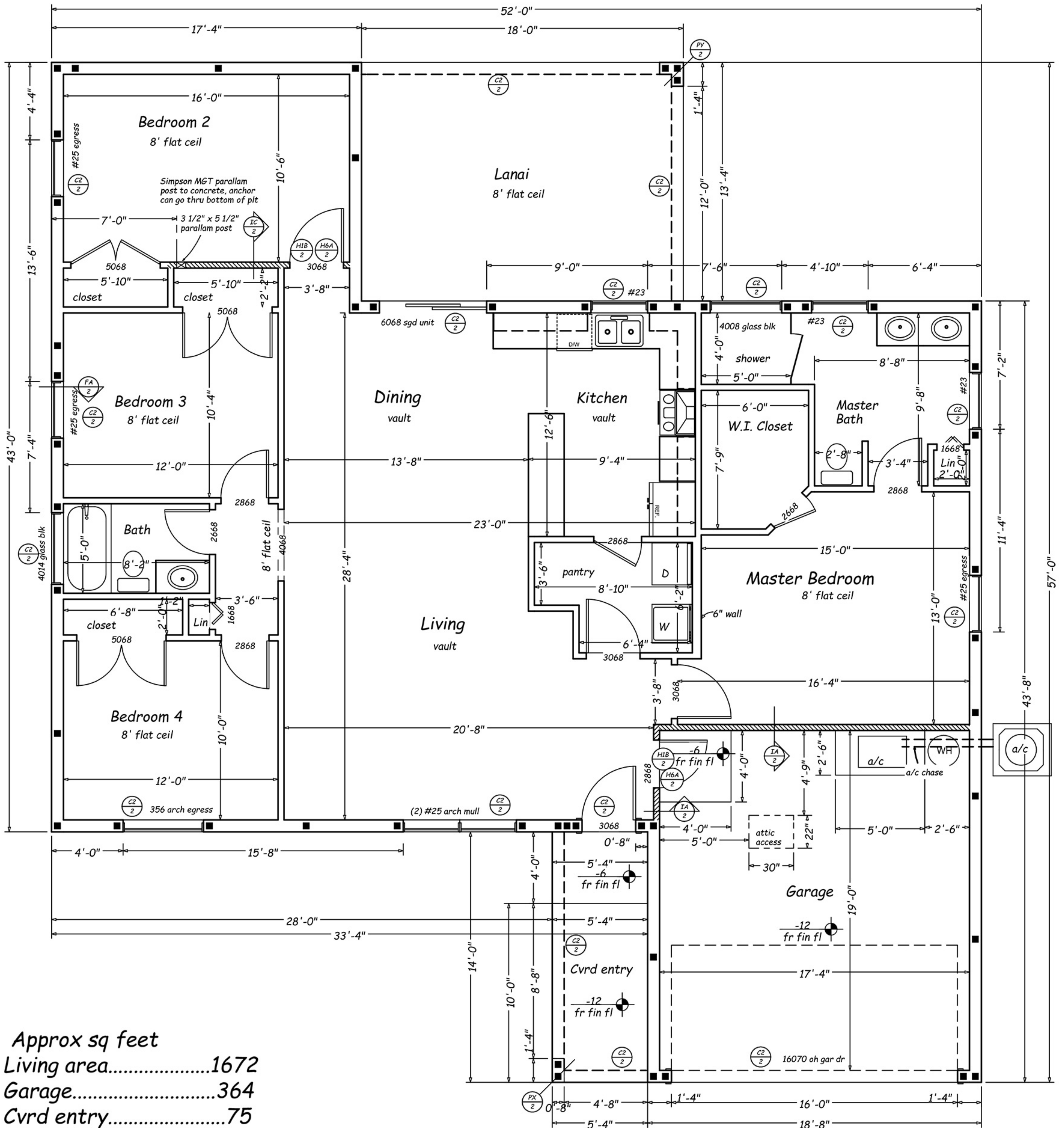
Floor Plan.....1/4"=1'0"
